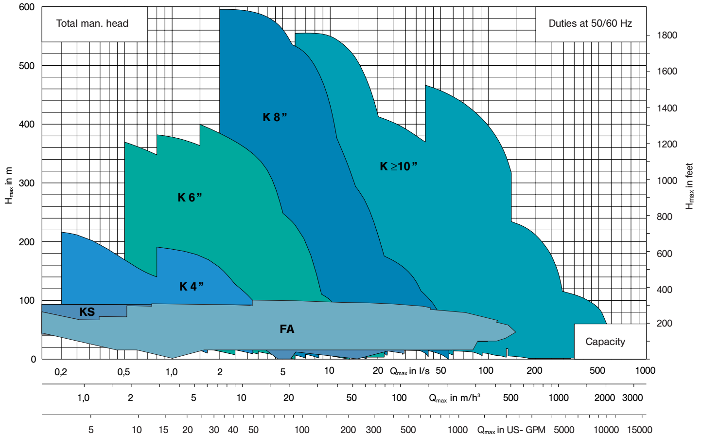
Performance curve
